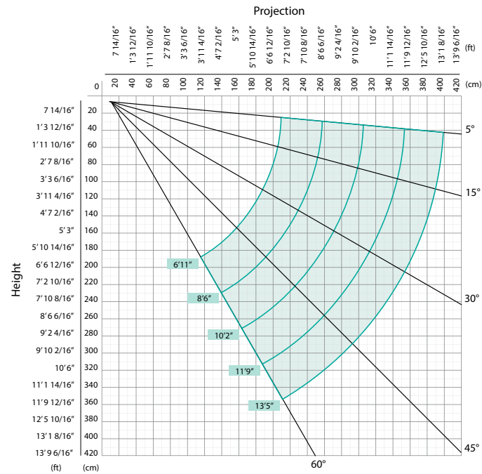
Covering diagram - Wall/ceiling installation
