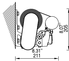
Wall installation
