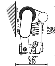
Crossed arms installation
